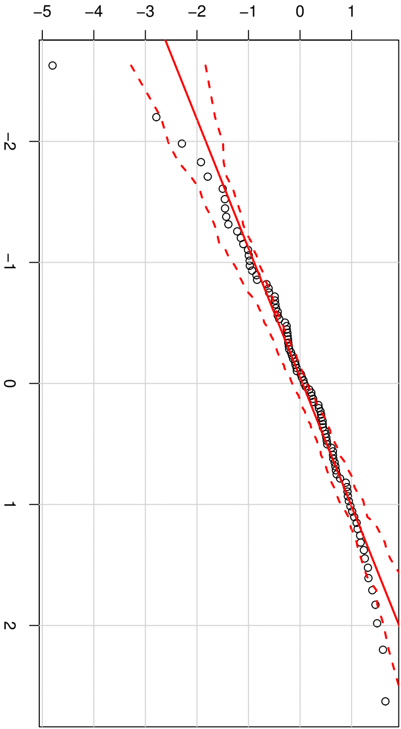
Studentized Residuals(mylm)
