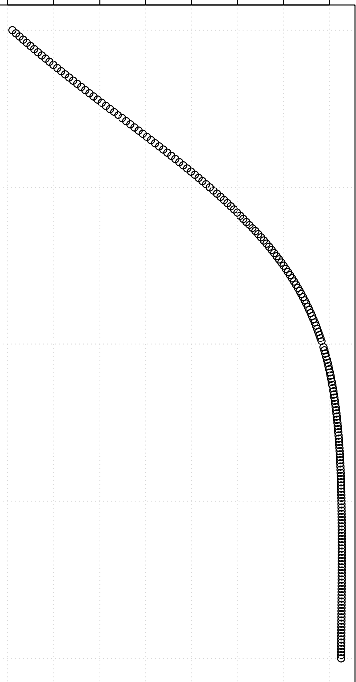
PPCC Plot – Tukey lambda
