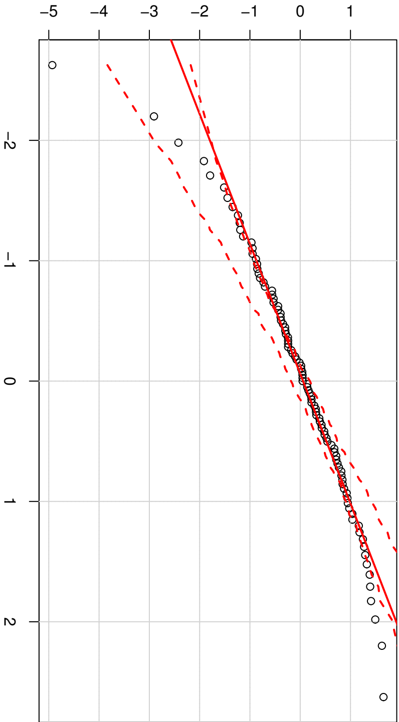
Studentized Residuals(myIm)
