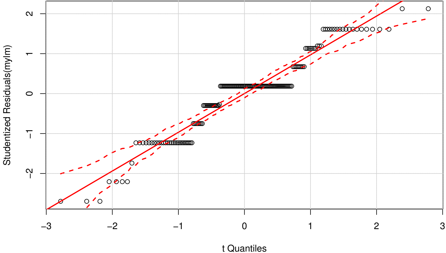
QQ Plot
