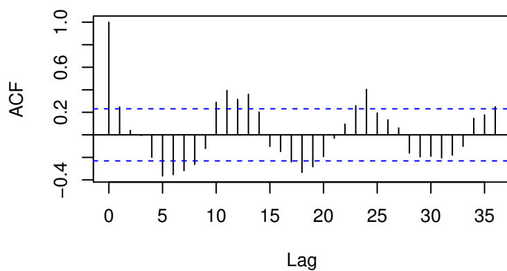
Standardized Residuals
