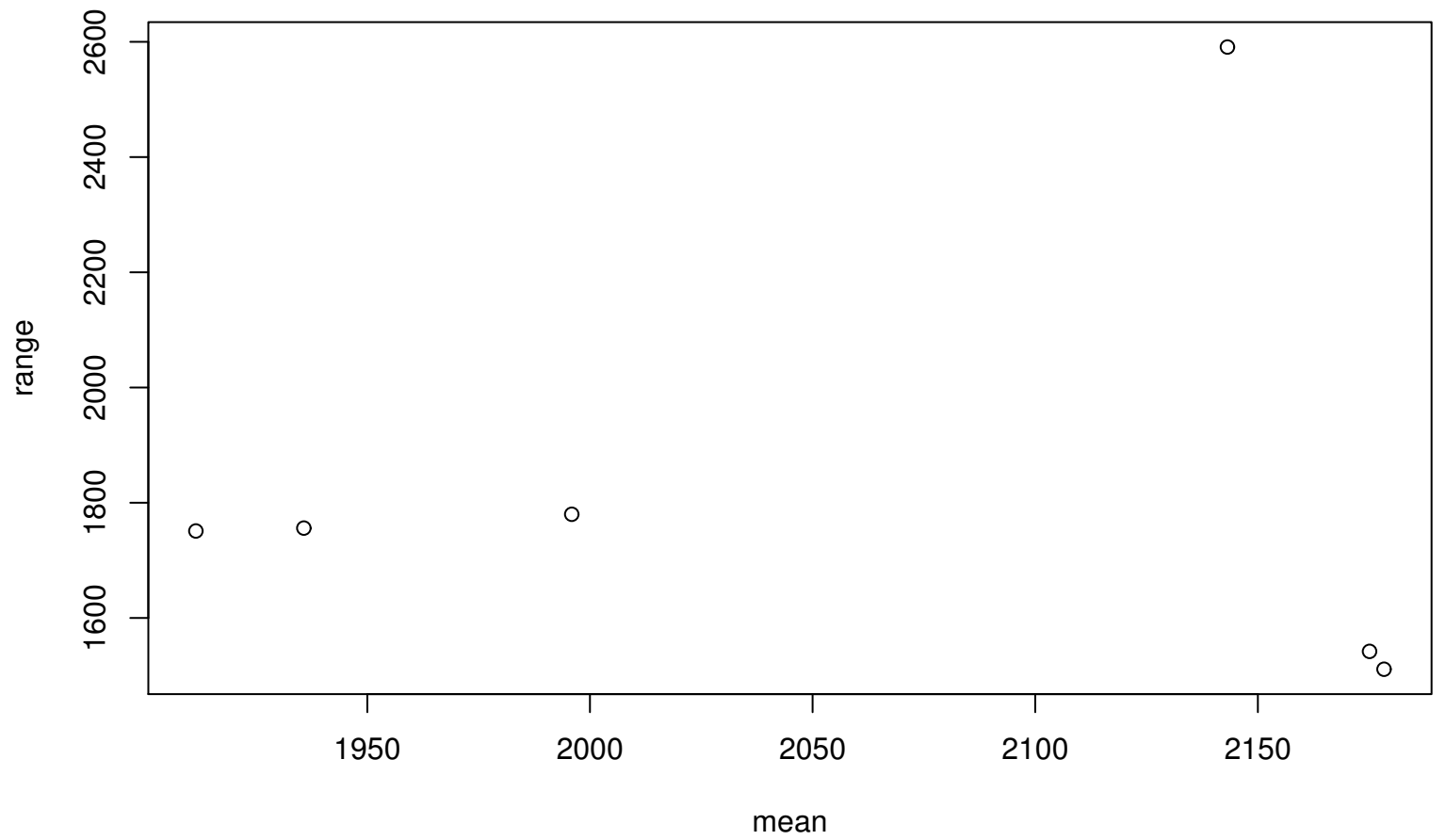
Range–Mean Plot
