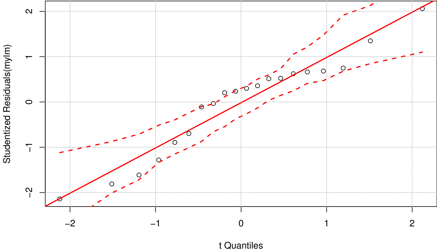
QQ Plot
