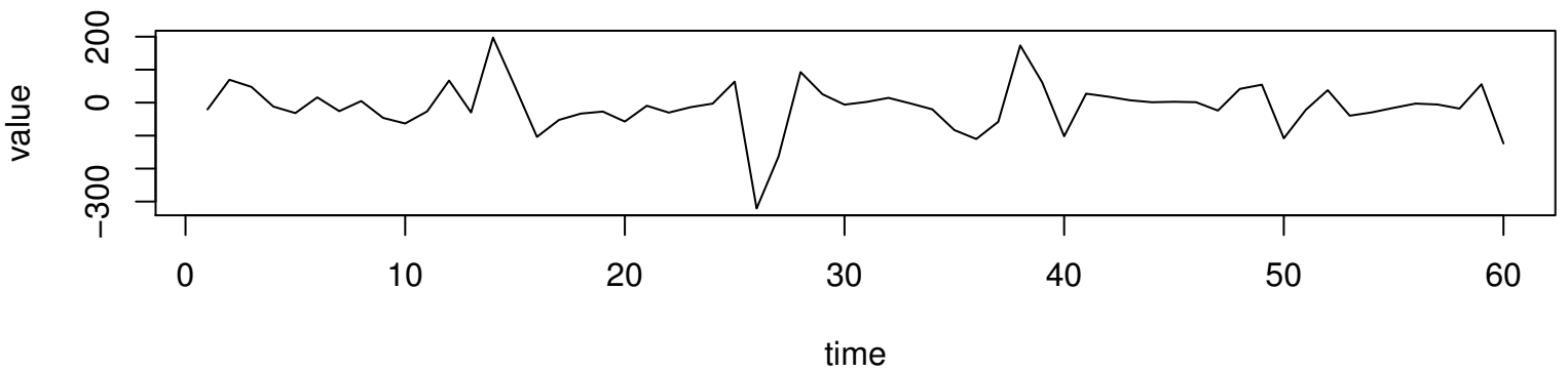
Working Time Series ( \lambda=0.8 , d=0 , D=1 )
