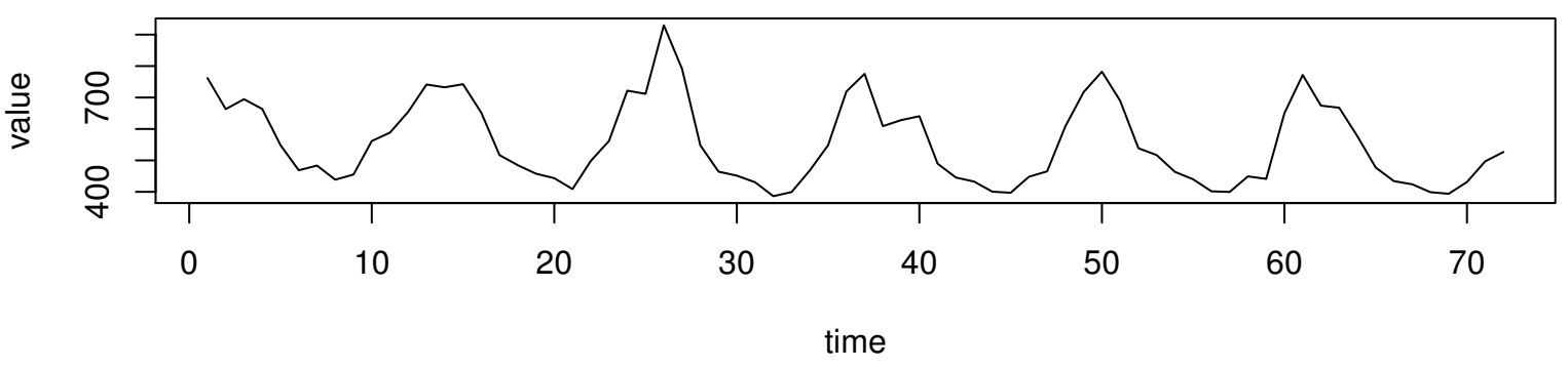
Working Time Series (lambda=0.8, d=0, D=0)
