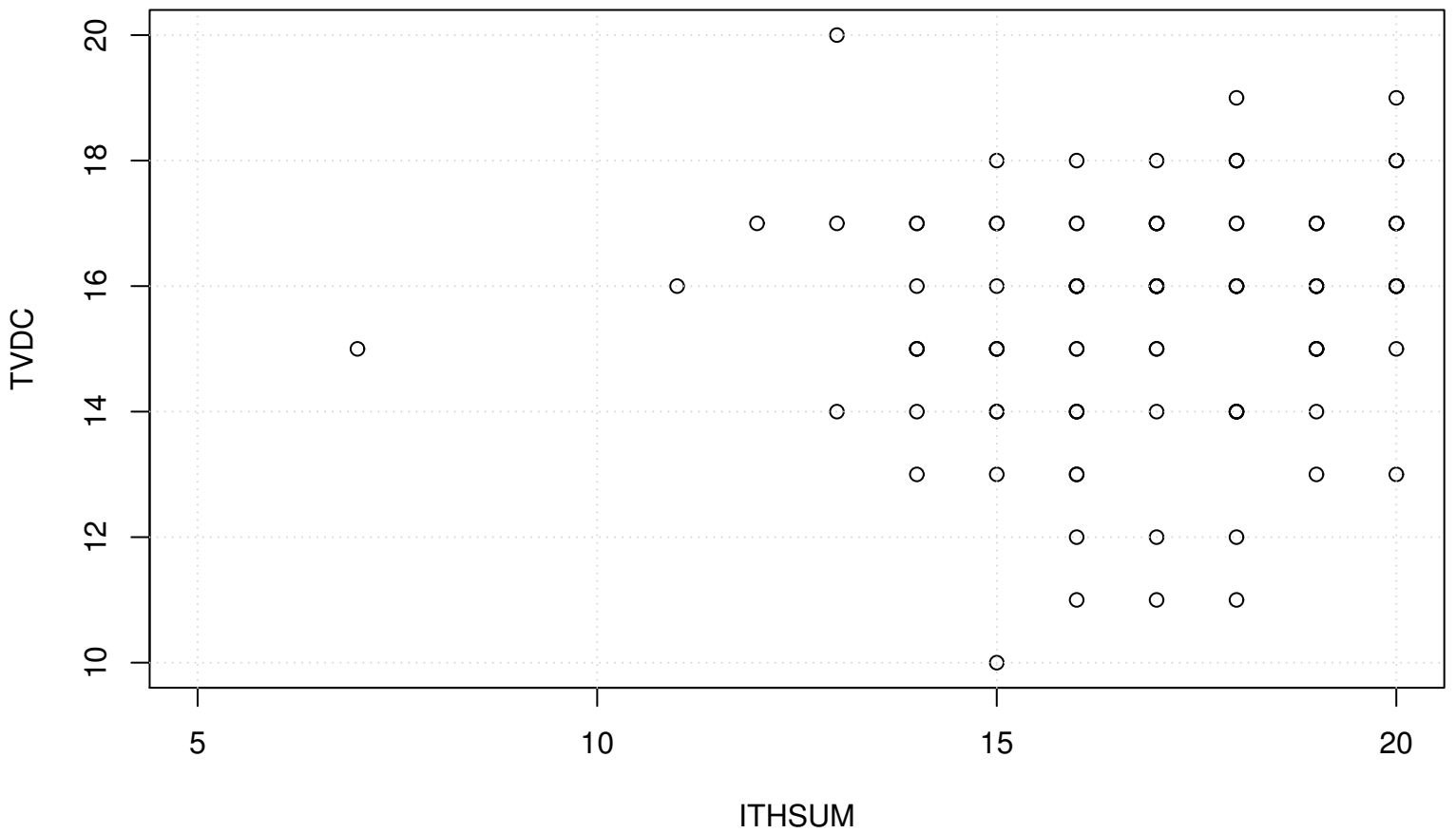
Scatterplot
