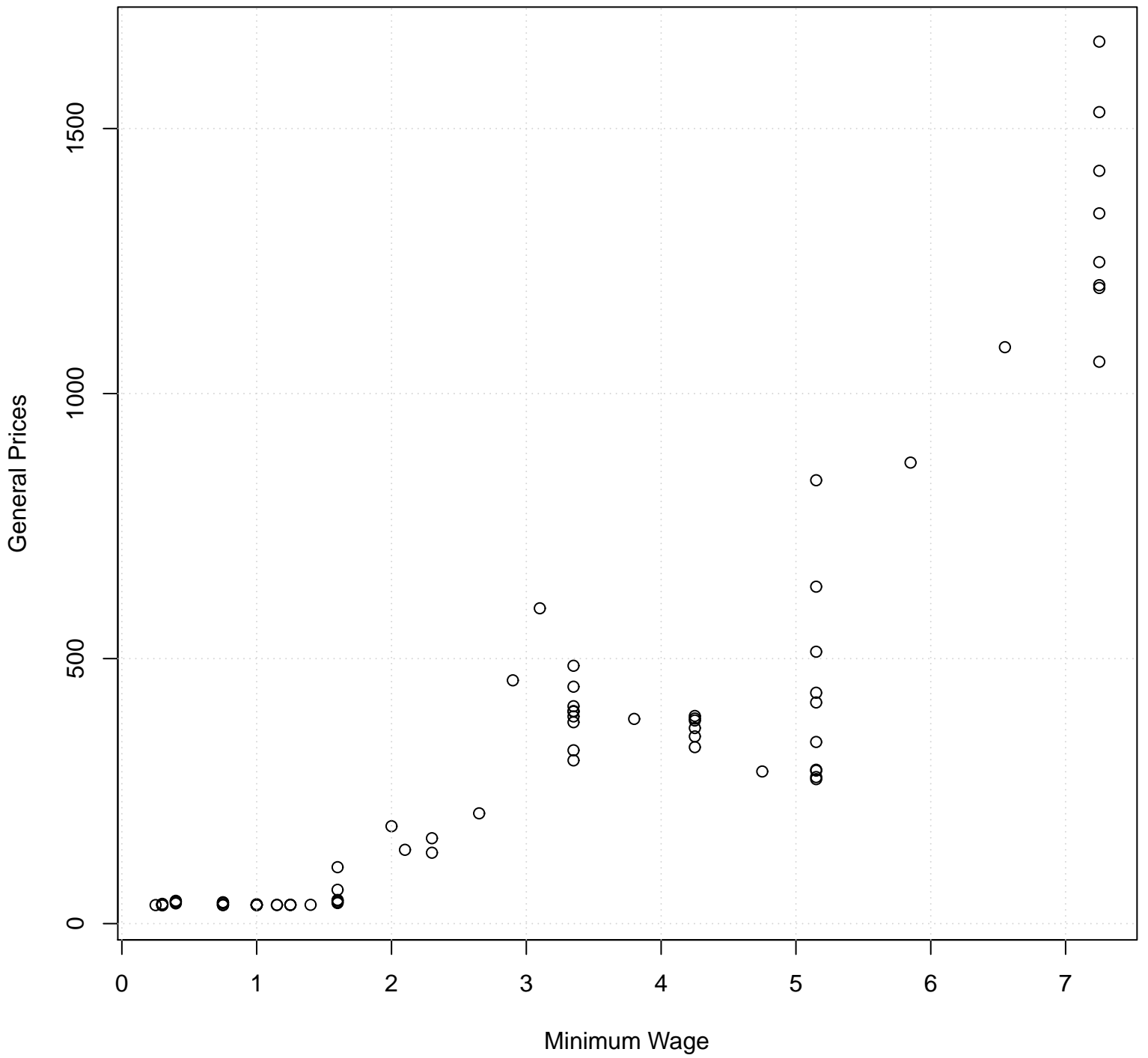
Scatterplot
