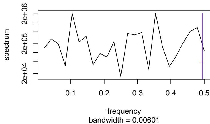
Random
