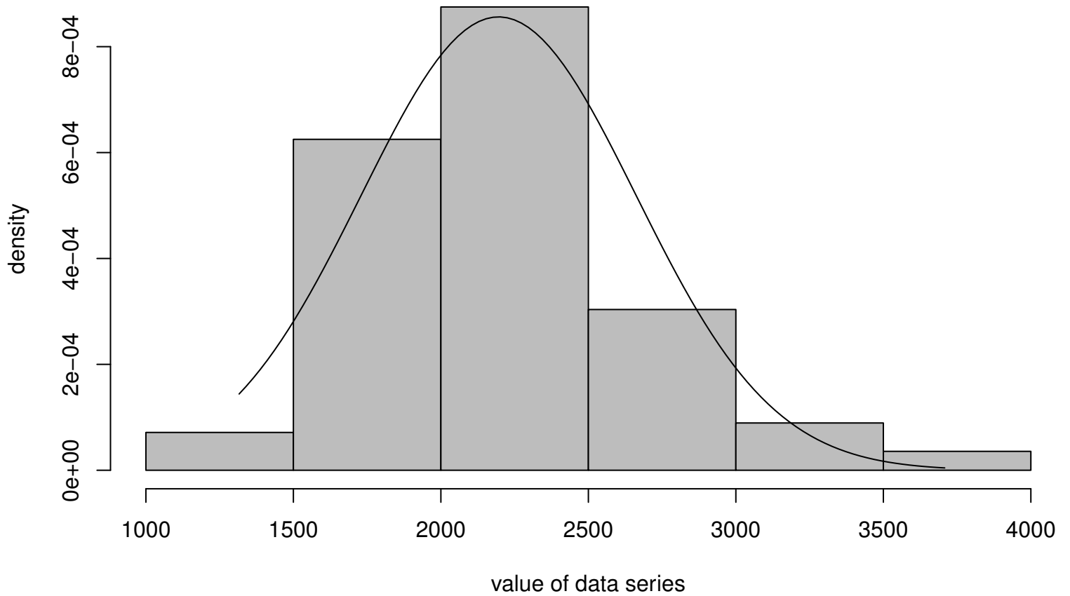
Histogram and Fitted Normal Density
