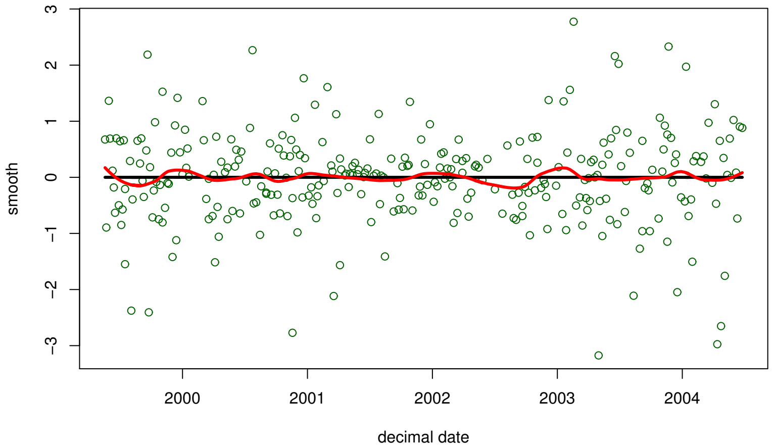
Residuals of (Data - Smooth)
