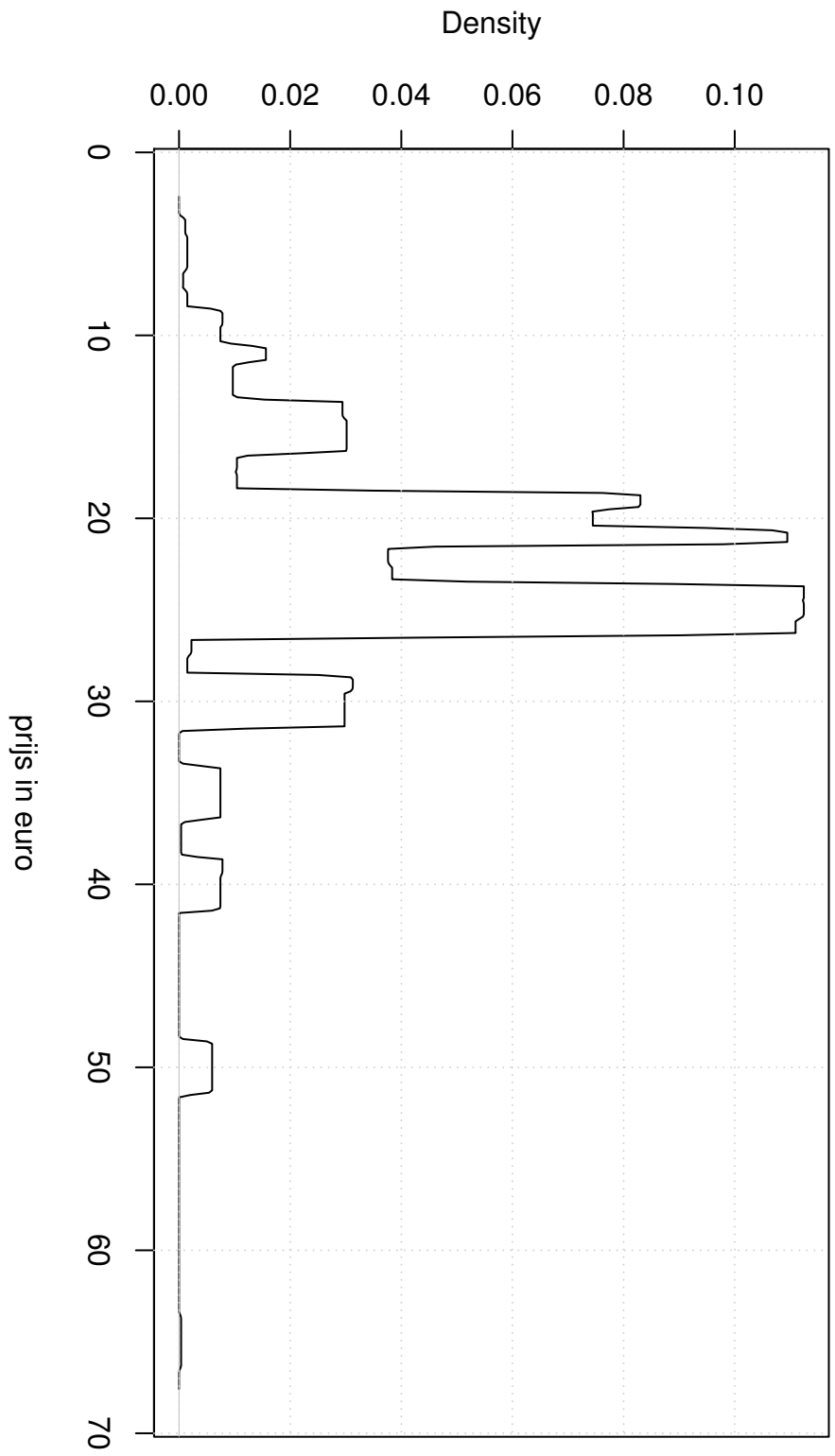
Rectangular Kernel
