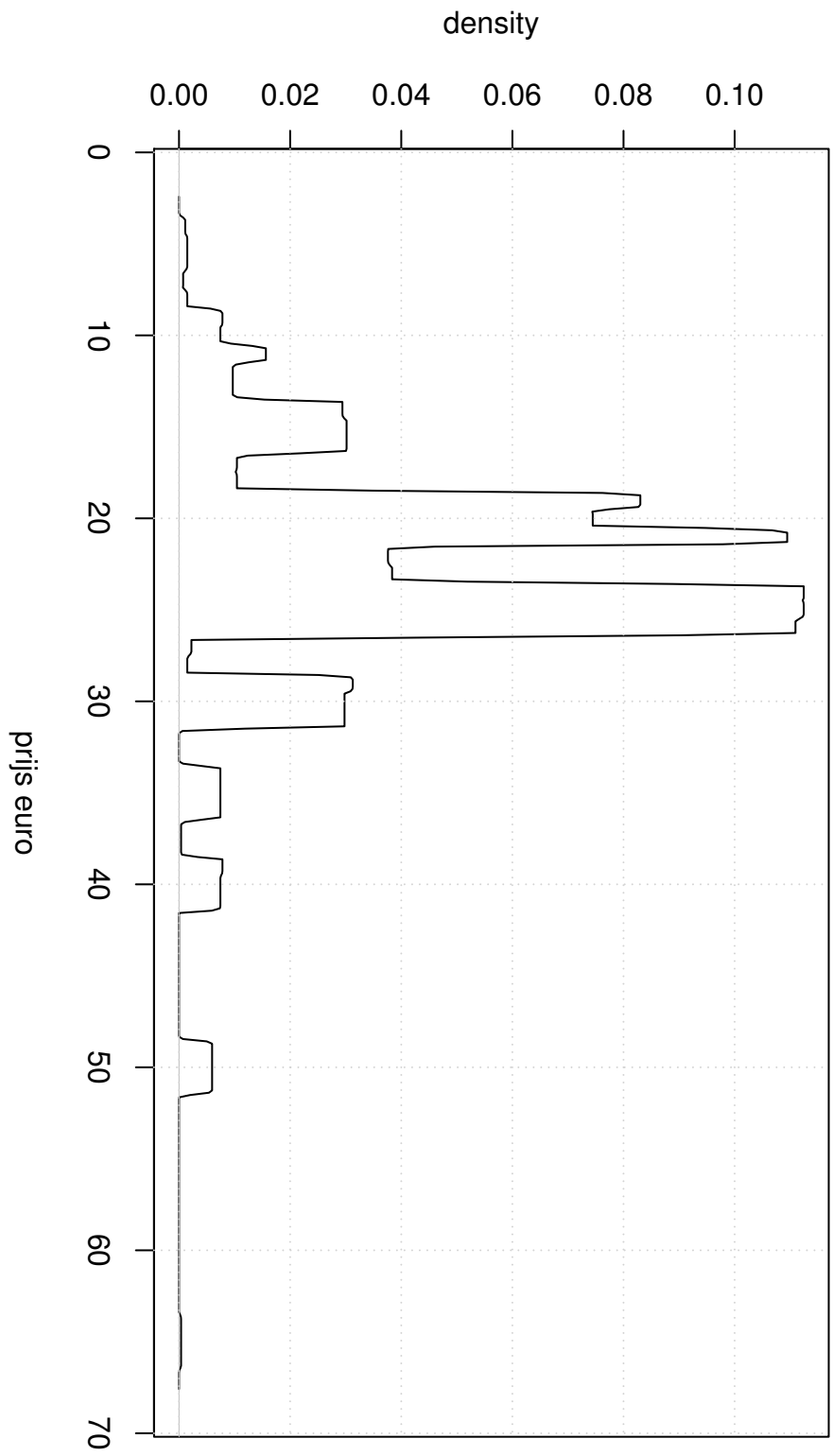
Rectangular Kernel
