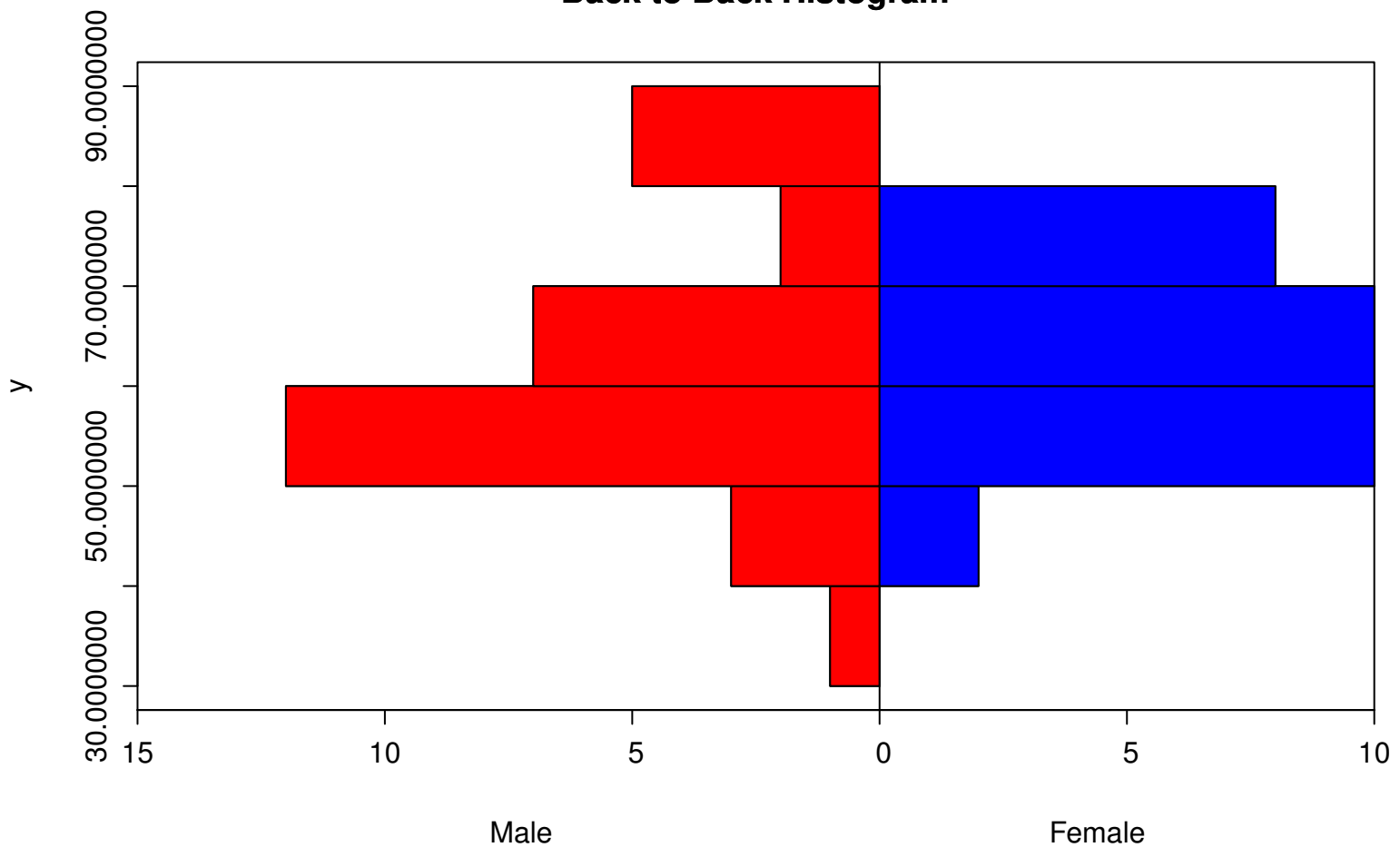
Back to Back Histogram
