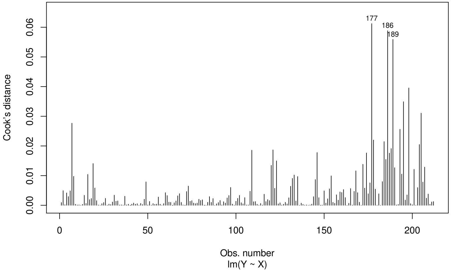
Cook's distance
