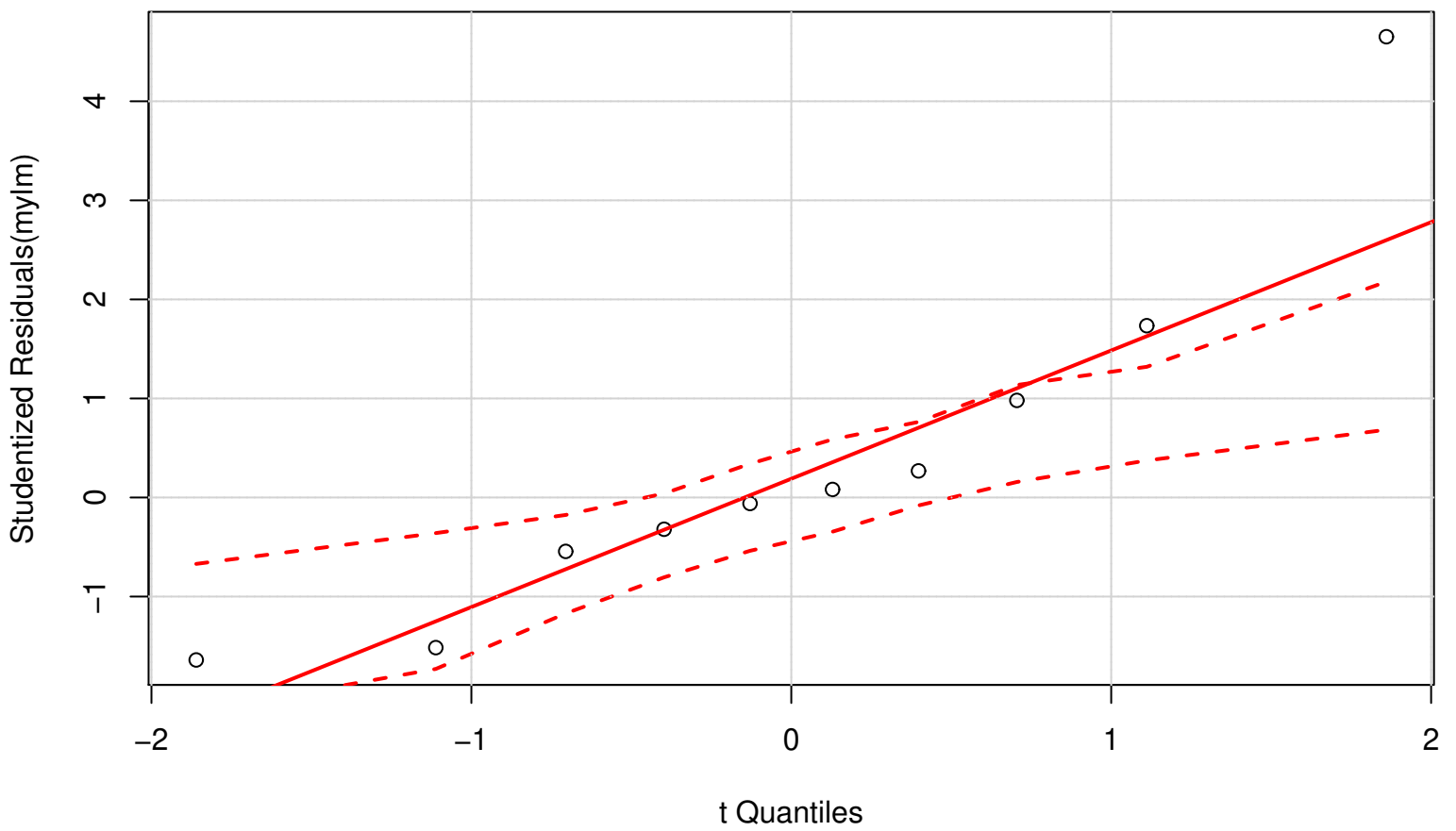
QQ Plot
