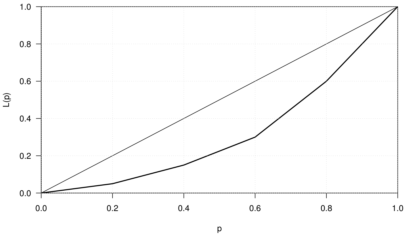
Lorenz curve
