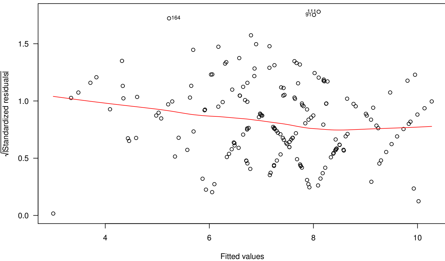
Scale-Location
