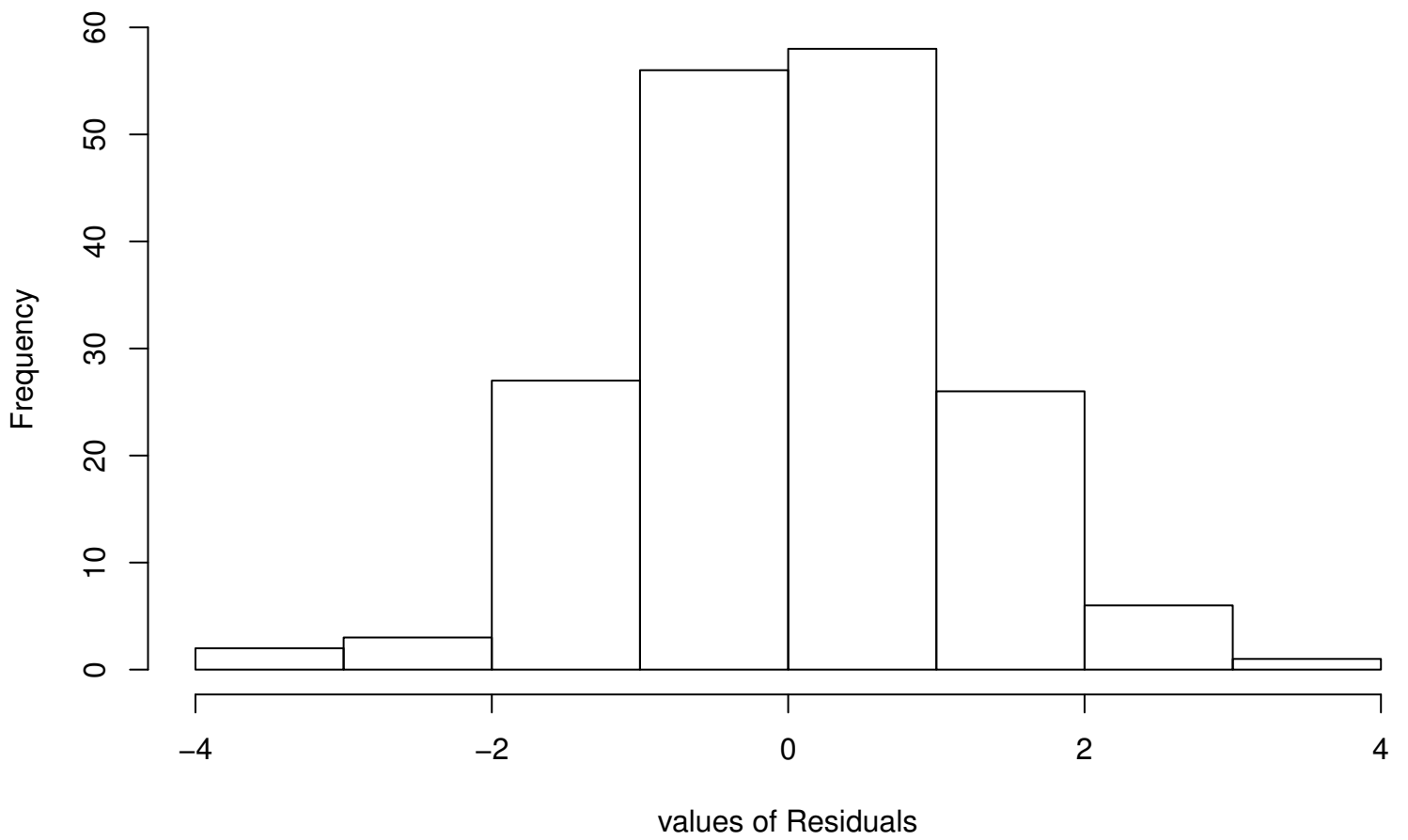
Residual Histogram
