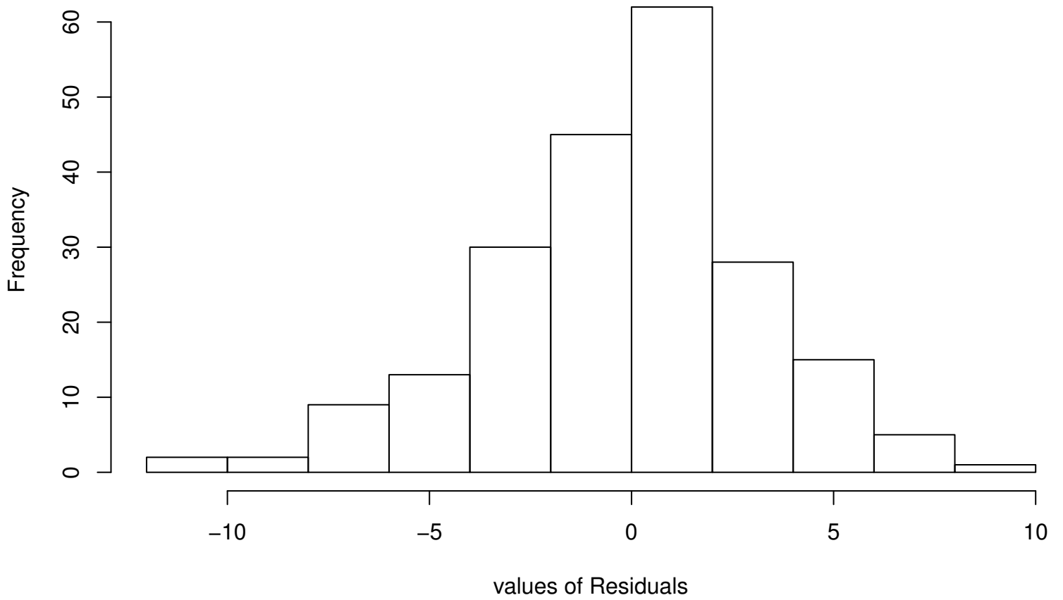
Residual Histogram
