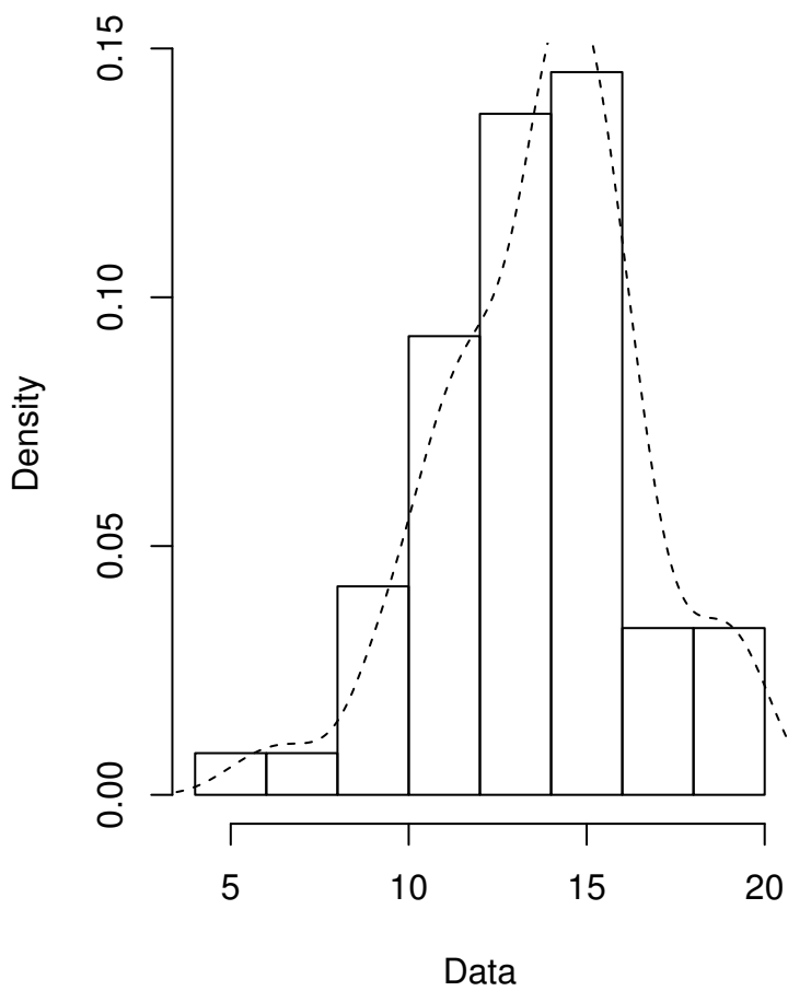
Empirical density
