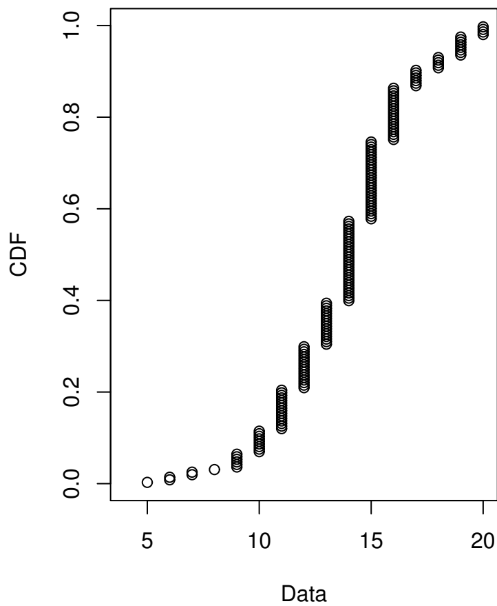
Cumulative distribution
