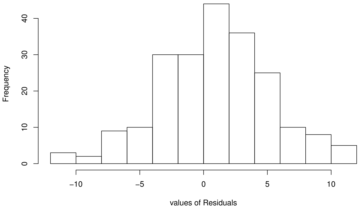
Residual Histogram
