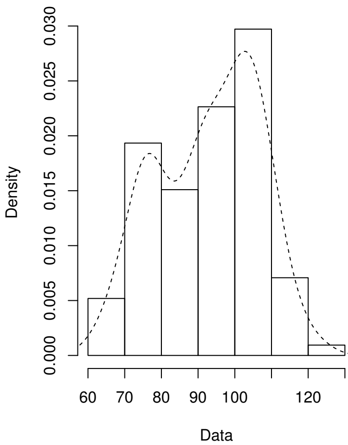
Empirical density
