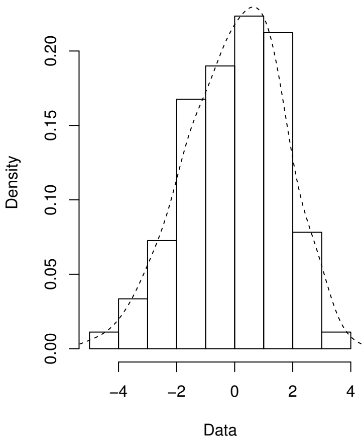
Empirical density
