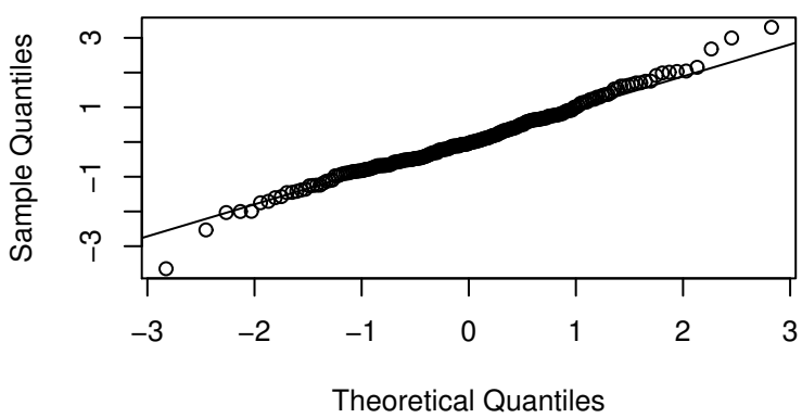
Residual Normal QQ Plot
