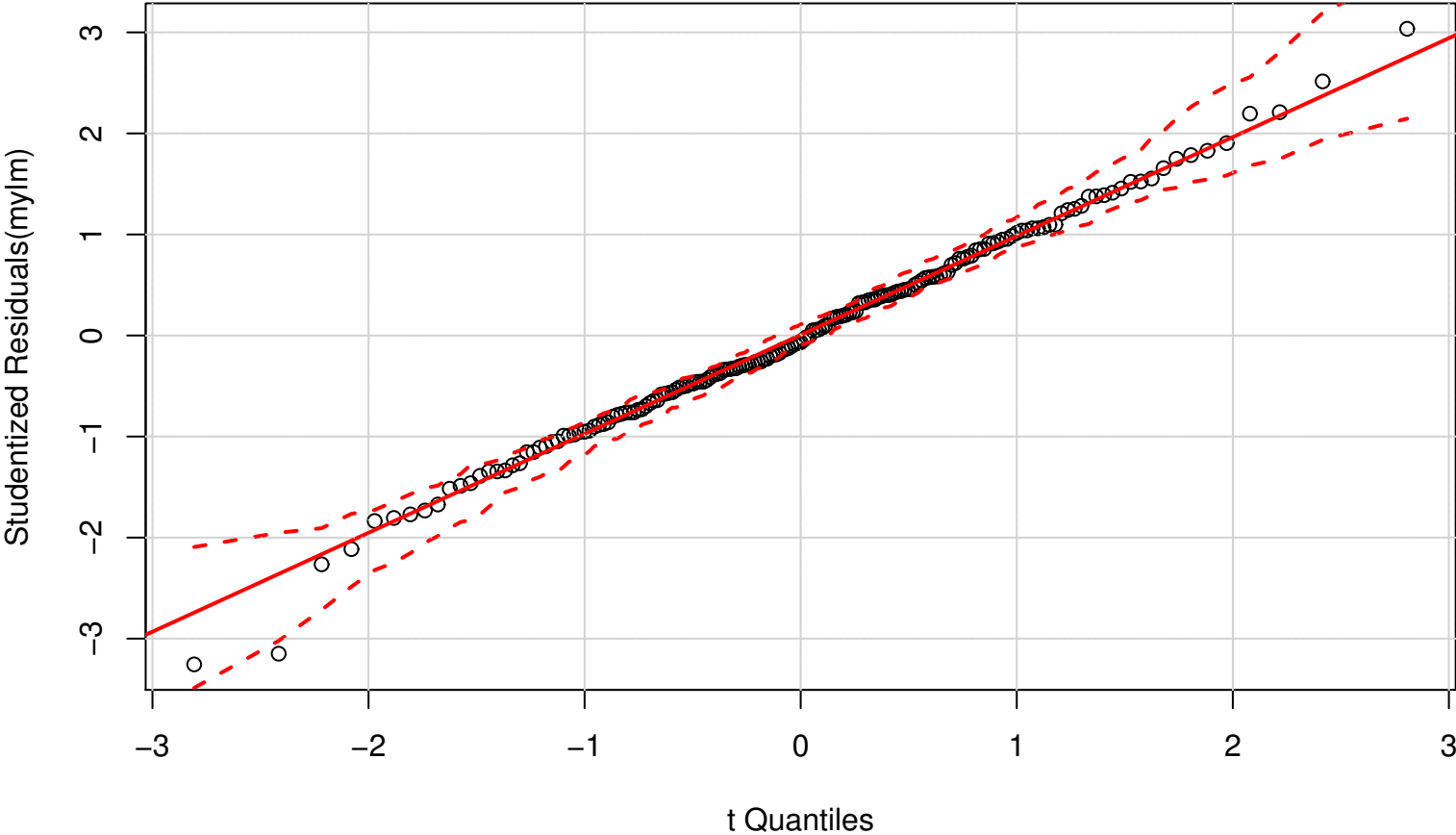
QQ Plot
