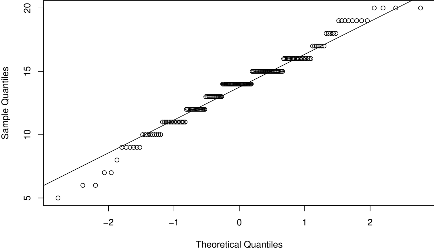
Normal QQplot – Variable 2
