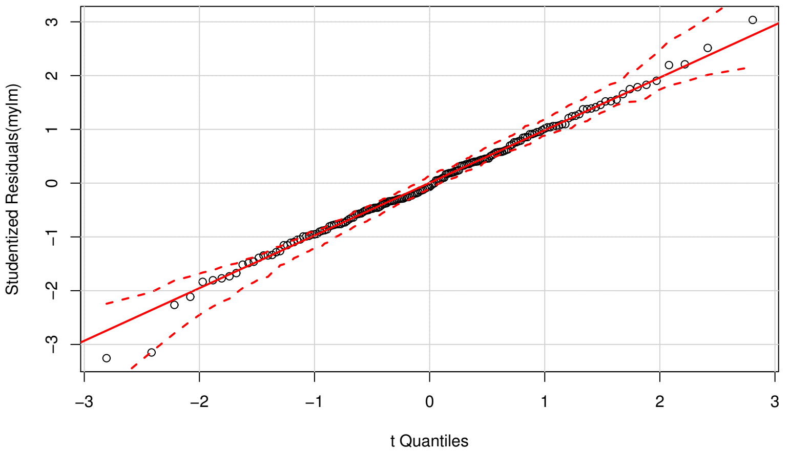
QQ Plot
