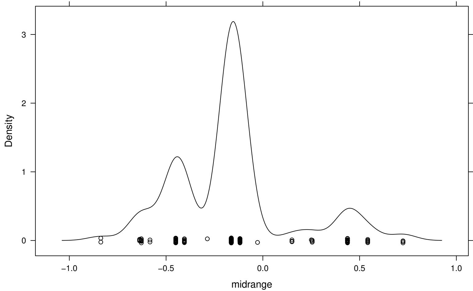
Density Plot
