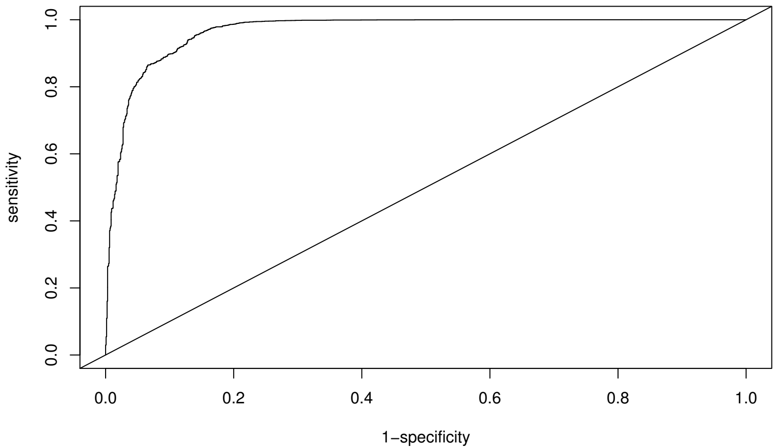
ROC plot
