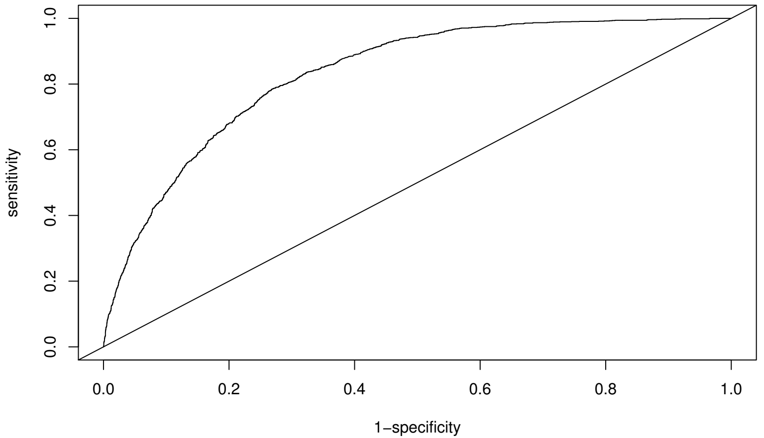
ROC plot
