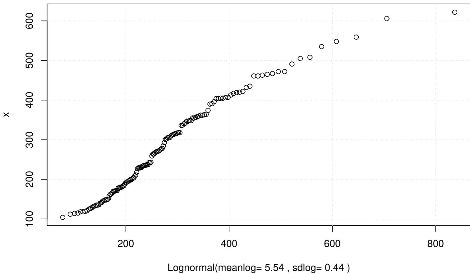
QQ plot (Lognormal)
