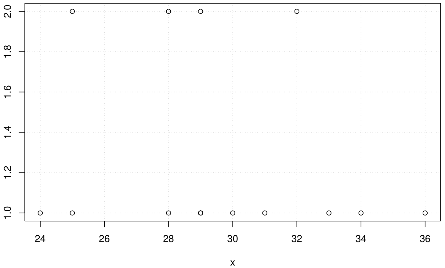
Scatterplot
