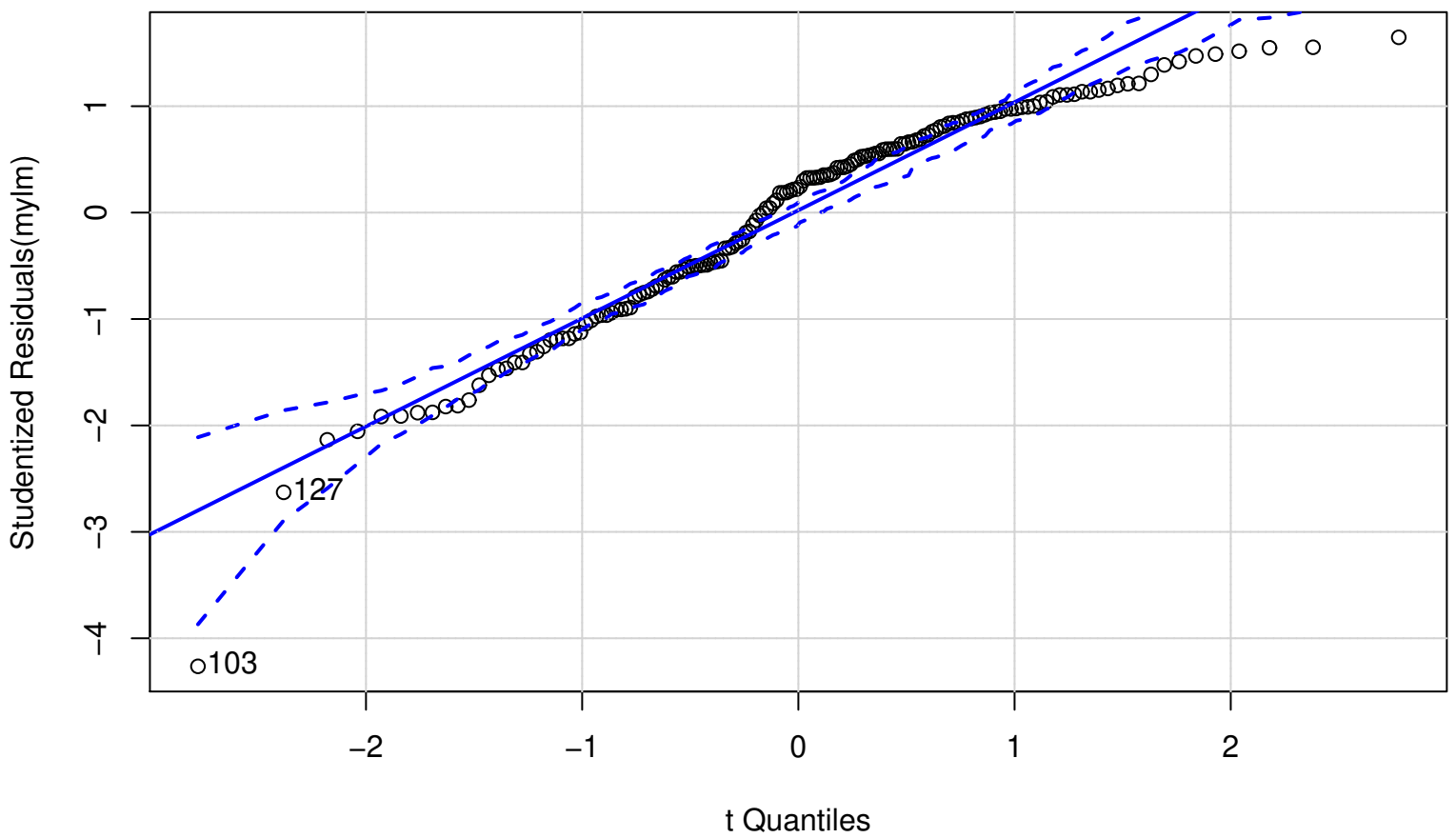
QQ Plot
