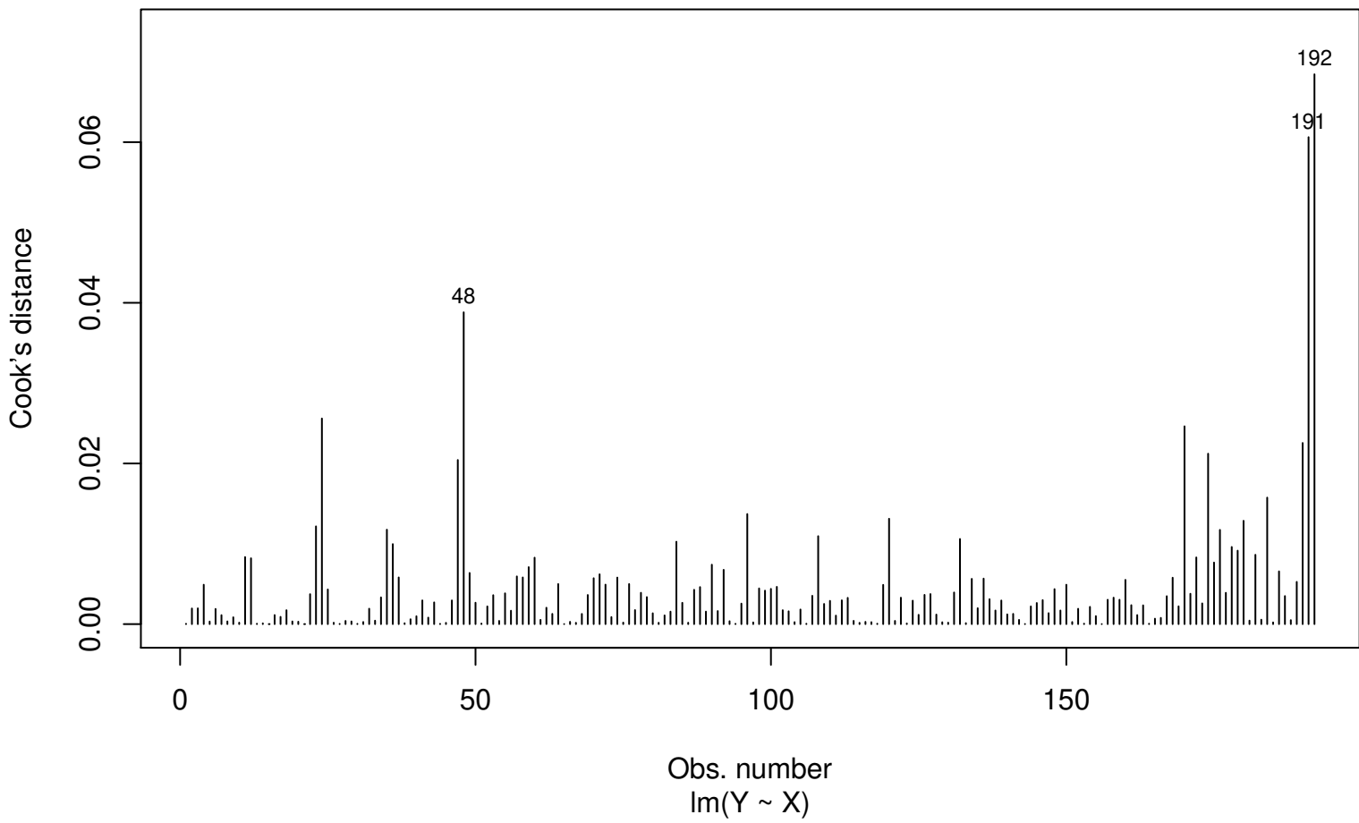
Cook's distance
