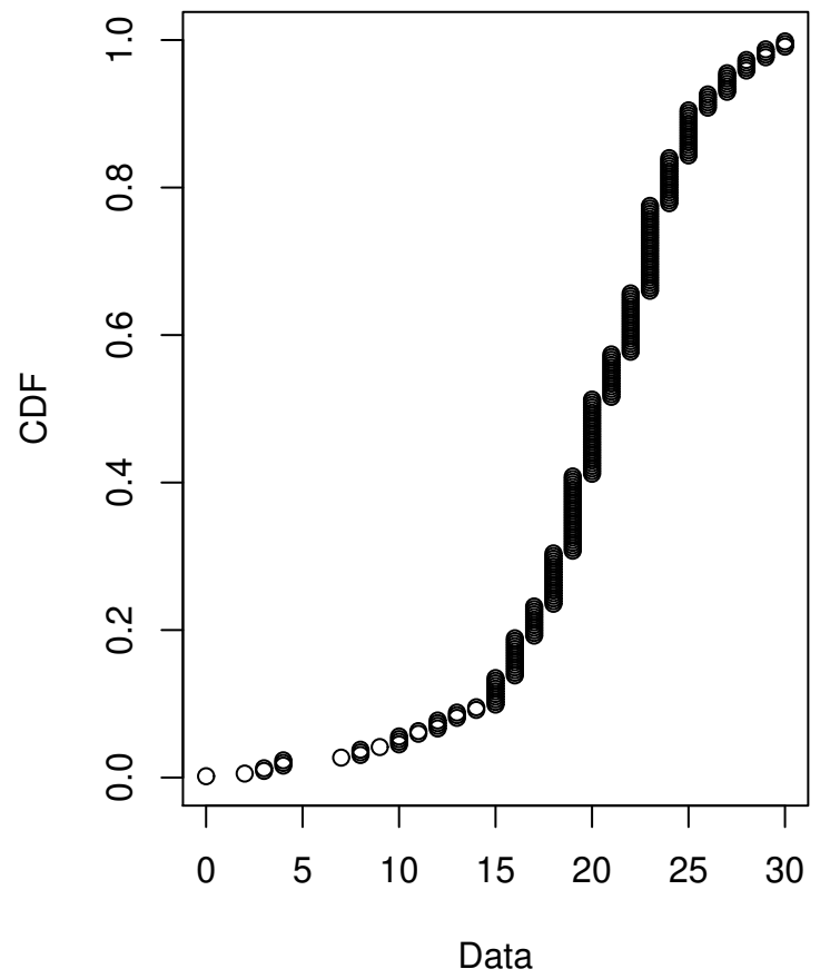
Cumulative distribution
