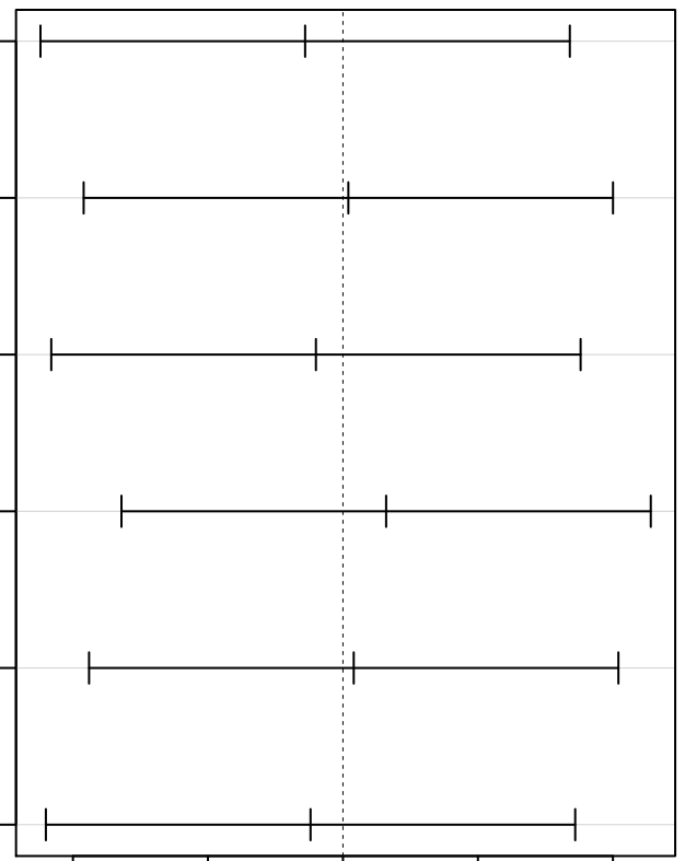
95% family-wise confidence level
