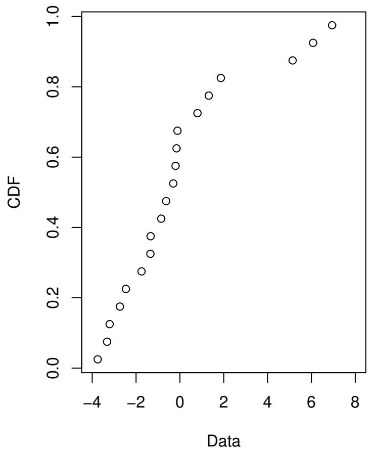
Cumulative distribution
