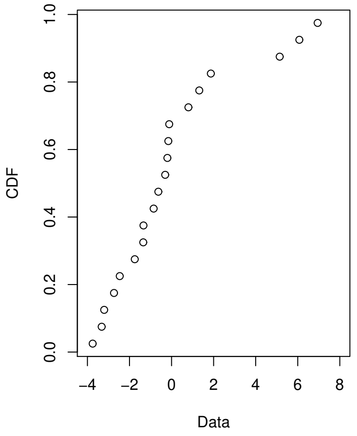
Cumulative distribution
