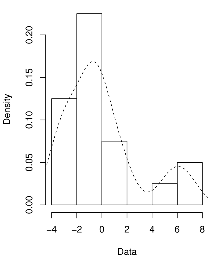
Empirical density
