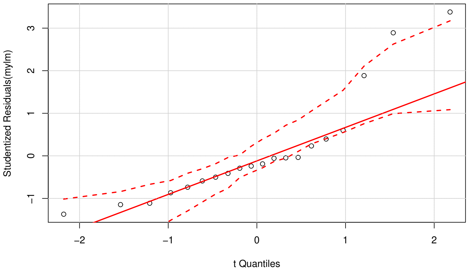
QQ Plot
