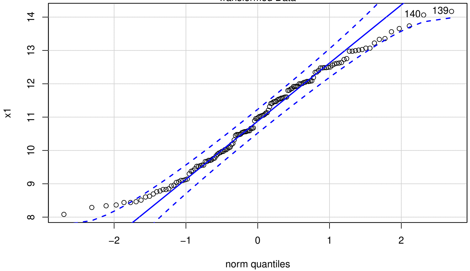
Transformed Data
