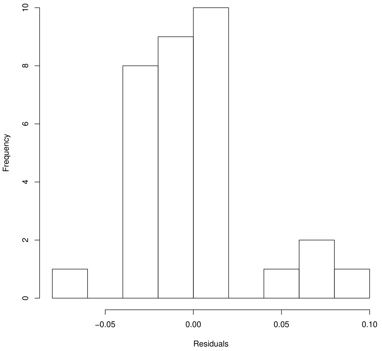
Residual Histogram
