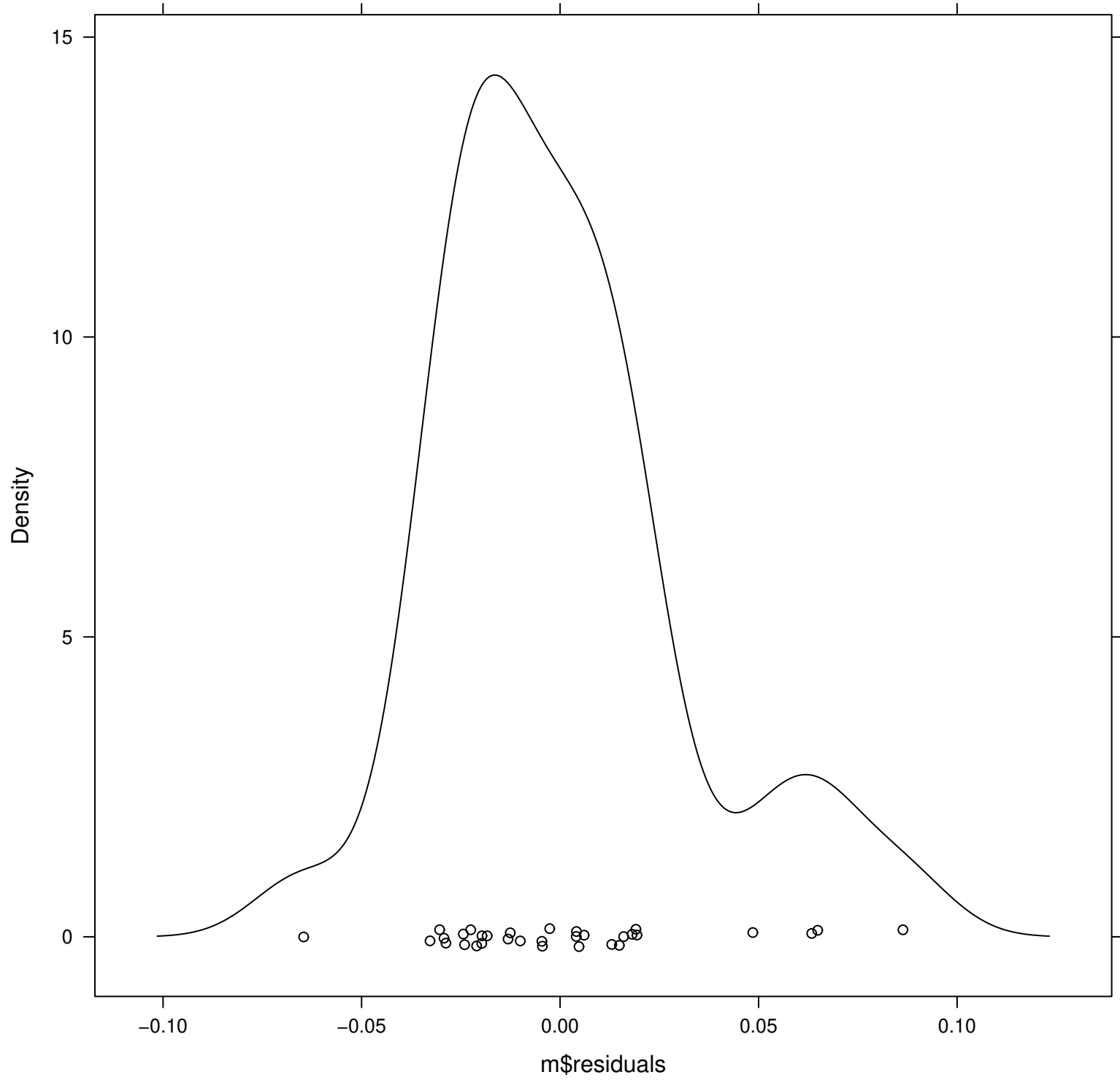
Density Plot
