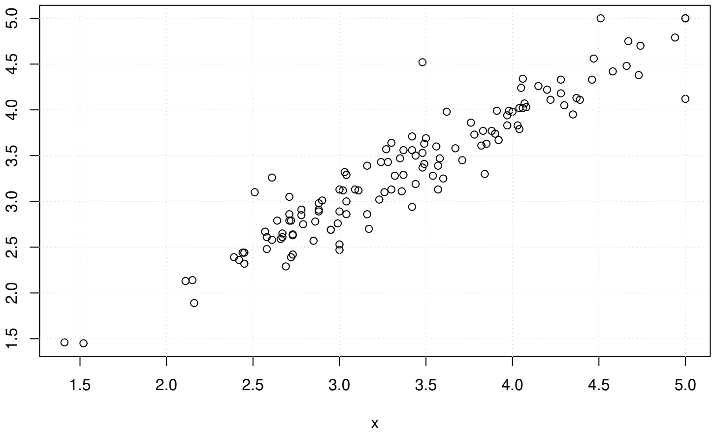
Scatterplot
