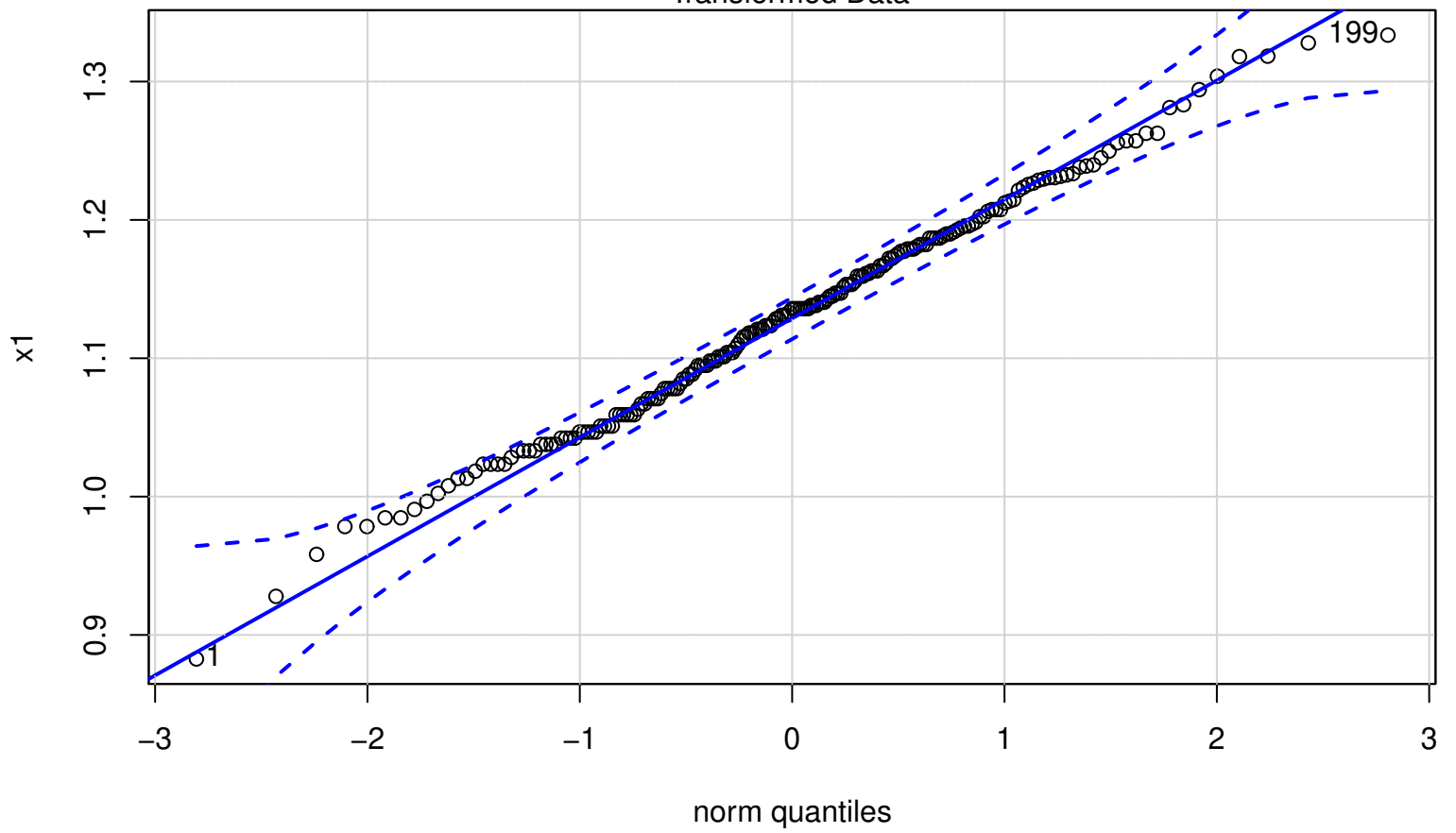
Transformed Data
