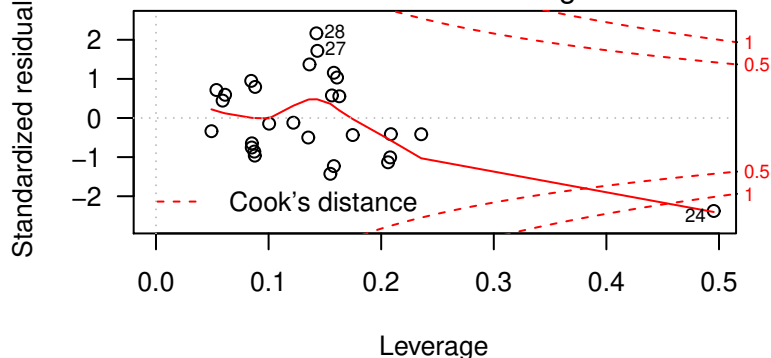
Residuals vs Leverage
