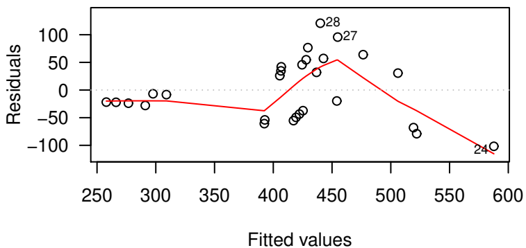
Residuals vs Fitted
