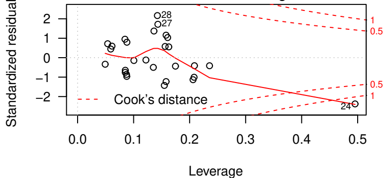
Residuals vs Leverage
